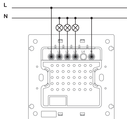
4-pole smart switch
