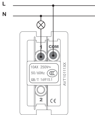
1gang 1-way switch
