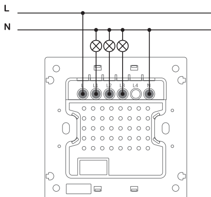
3-pole smart switch
