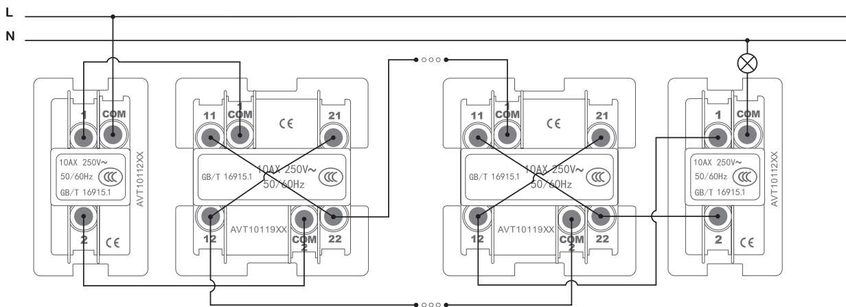
Two 1-gang 2-way switches + Two or more intermediate switches.
