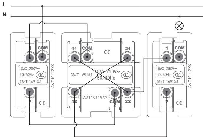
Two 1-gang 2-way switches + One intermediate switch.
