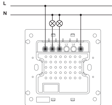
2-pole smart switch
