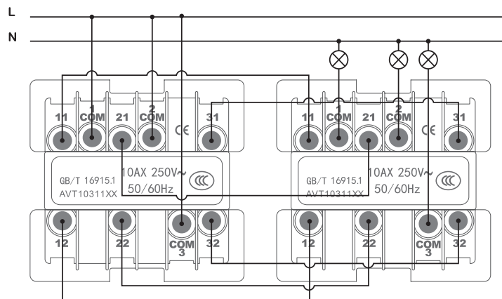
1gang 2-way switch
