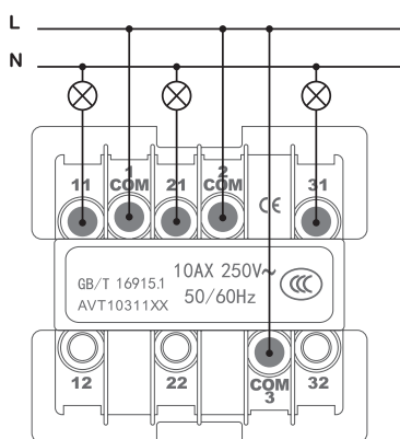
1gang 1-way switch
