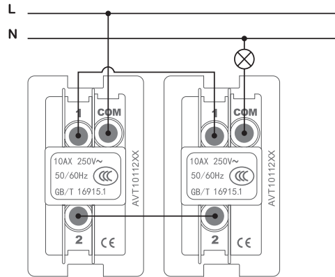
1gang 2-way switch
