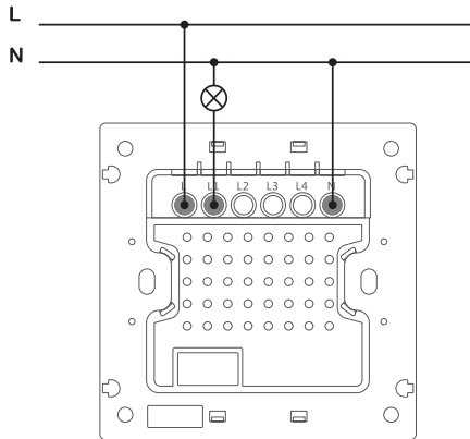
1-pole smart switch
