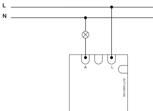
Dimmer switch
