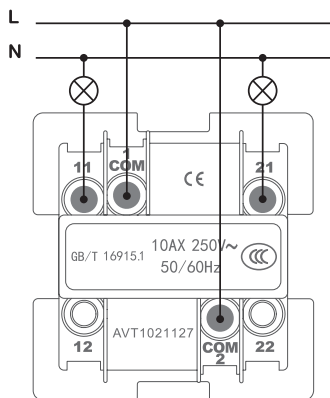
2-gang 1-way switch
