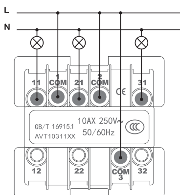
3-gang 1-way switch
