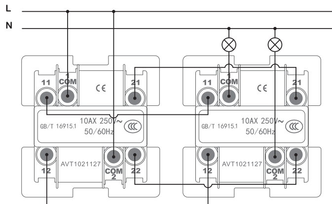
2-gang 2-way switch
